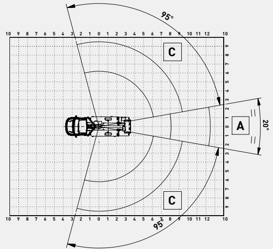
Scorpion 18 on Iveco P 3750 - Front outriggers opened 1 side only
