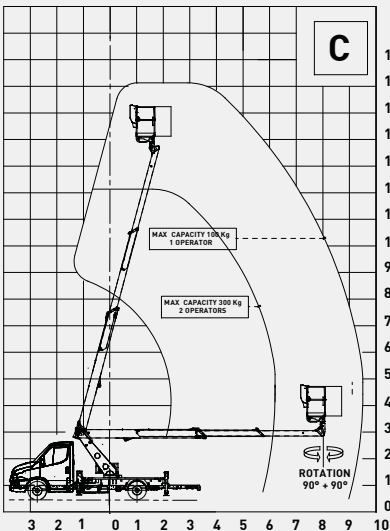
Scorpion 18 on Iveco P 3750 - Front outriggers opened 1 side only
