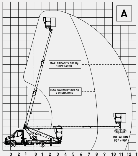
Scorpion 18 on Iveco P 3750 - Front outriggers opened 1 side only
