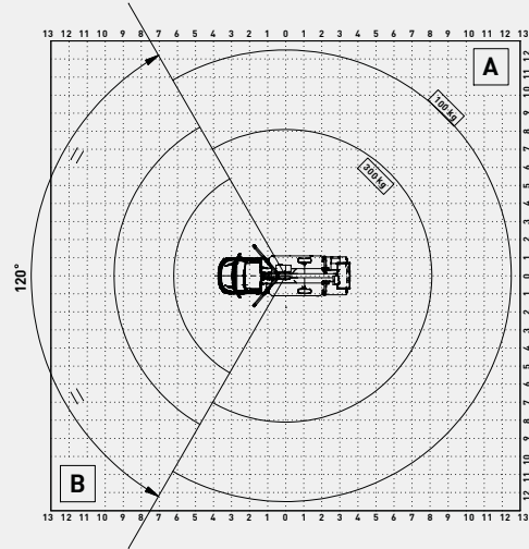
Scorpion 18 on Iveco P 3750 - Front outriggers closed
